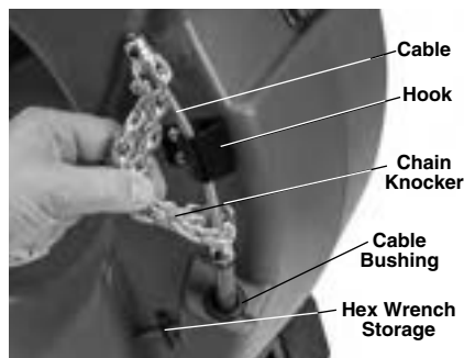
Figure 1C – Cable End/Chain Knocker
